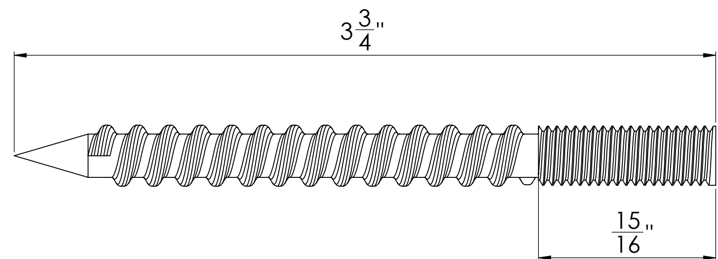
Hanger Bolt
