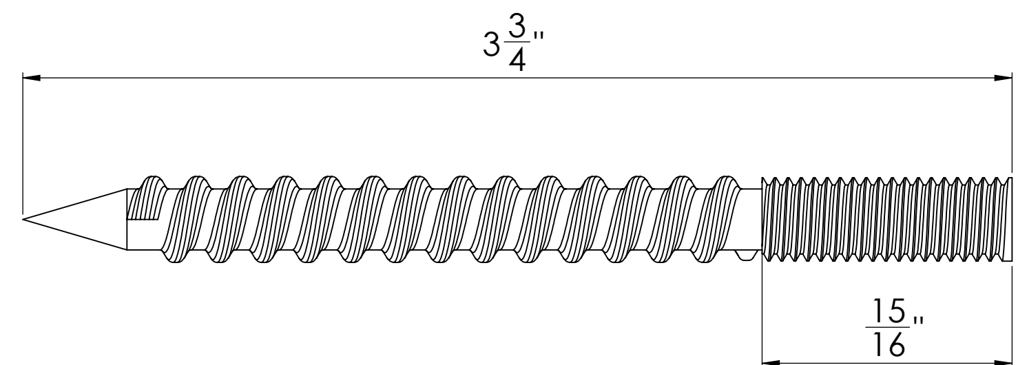
Hanger Bolt
