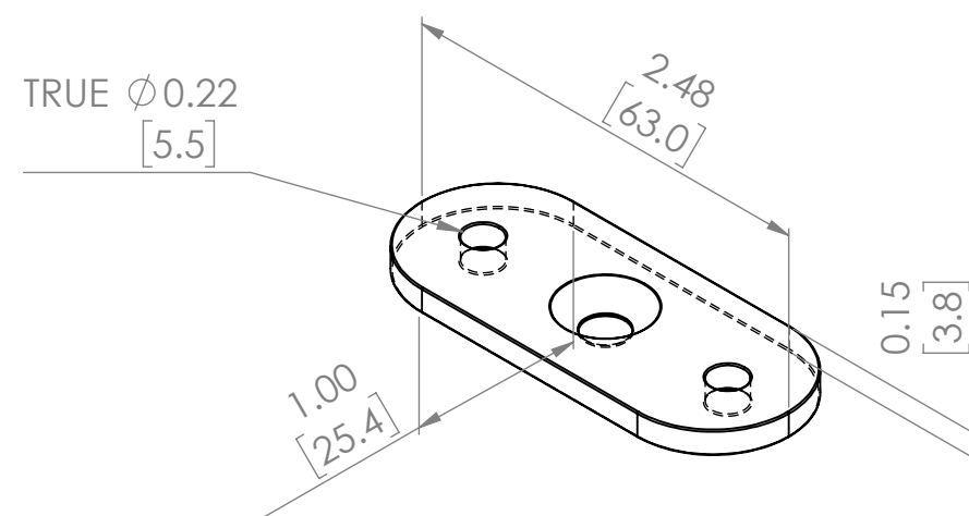
FLAT SADDLE OPTION
