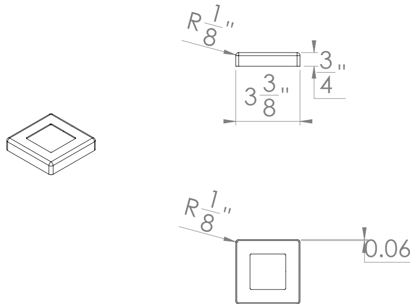
Base Cover
